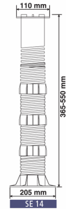
ETERNO ADJUSTABLE PAVING SUPPORT WITH SELF LEVELING HEAD
