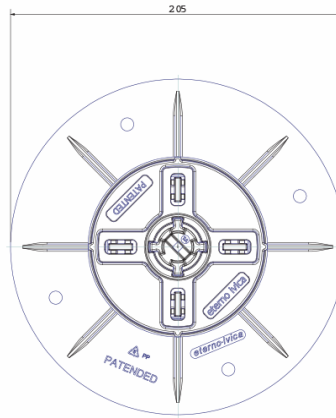
ETERNO ADJUSTABLE PAVING SUPPORT WITH SELF LEVELING HEAD
